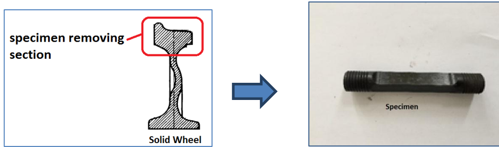
Figure 1. Wheel Cutting
