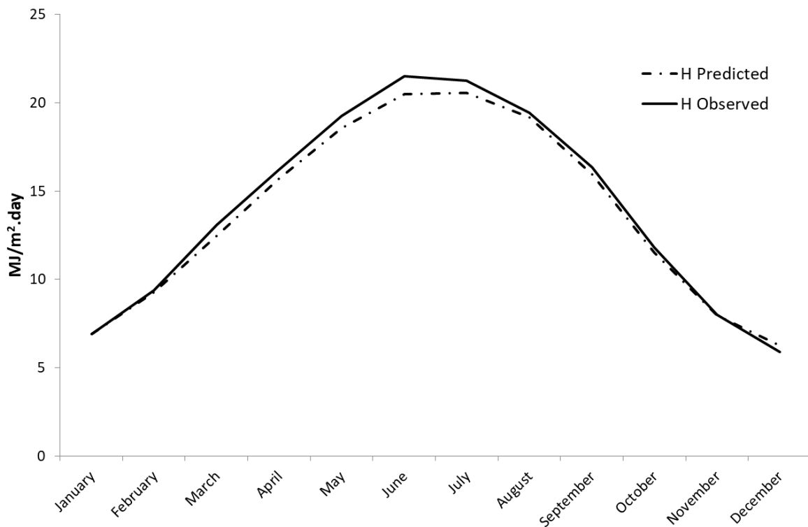
Figure 3. Observed and predicted global solar radiation by Model 1
