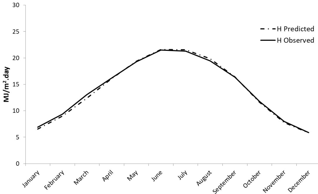
Figure 6. Observed and predicted global solar radiation by Model 4
